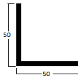
600867 ANGULAR 50x50x2mm
