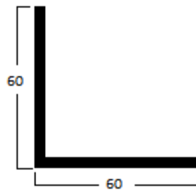
1102 ANGULAR 60x60x2mm
