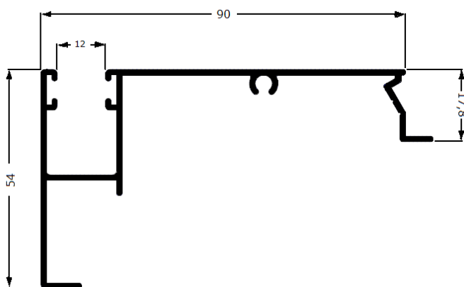
CMD3776 GUIA MONOBLOCK DE 90 mm
