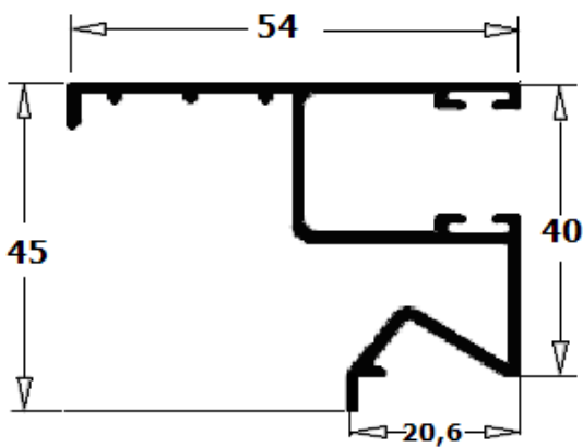
74993 GUIA PERSIANA DE 40mm
